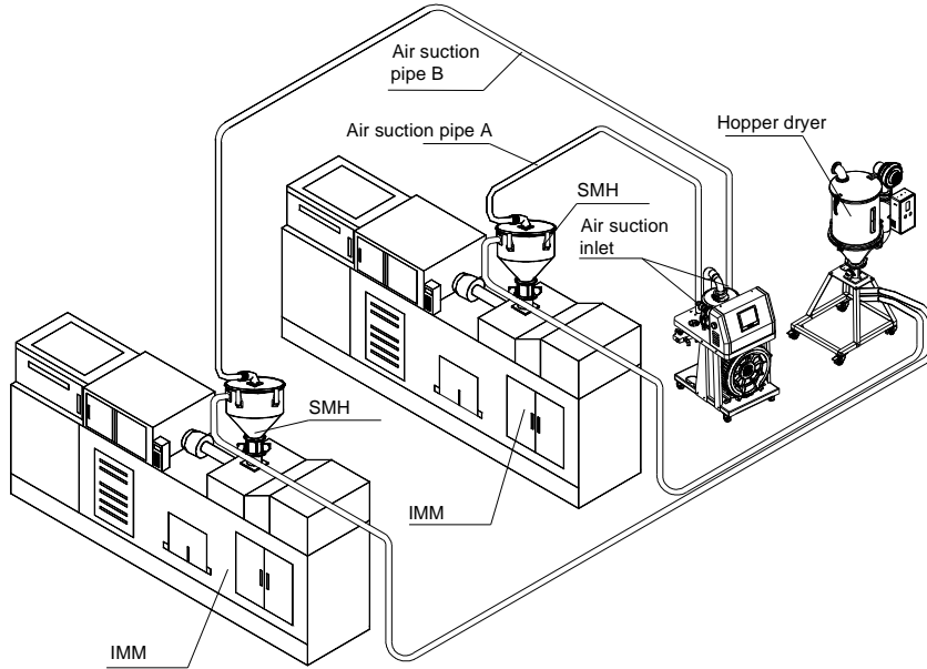
Picture 3-3: Installation Layout 2
