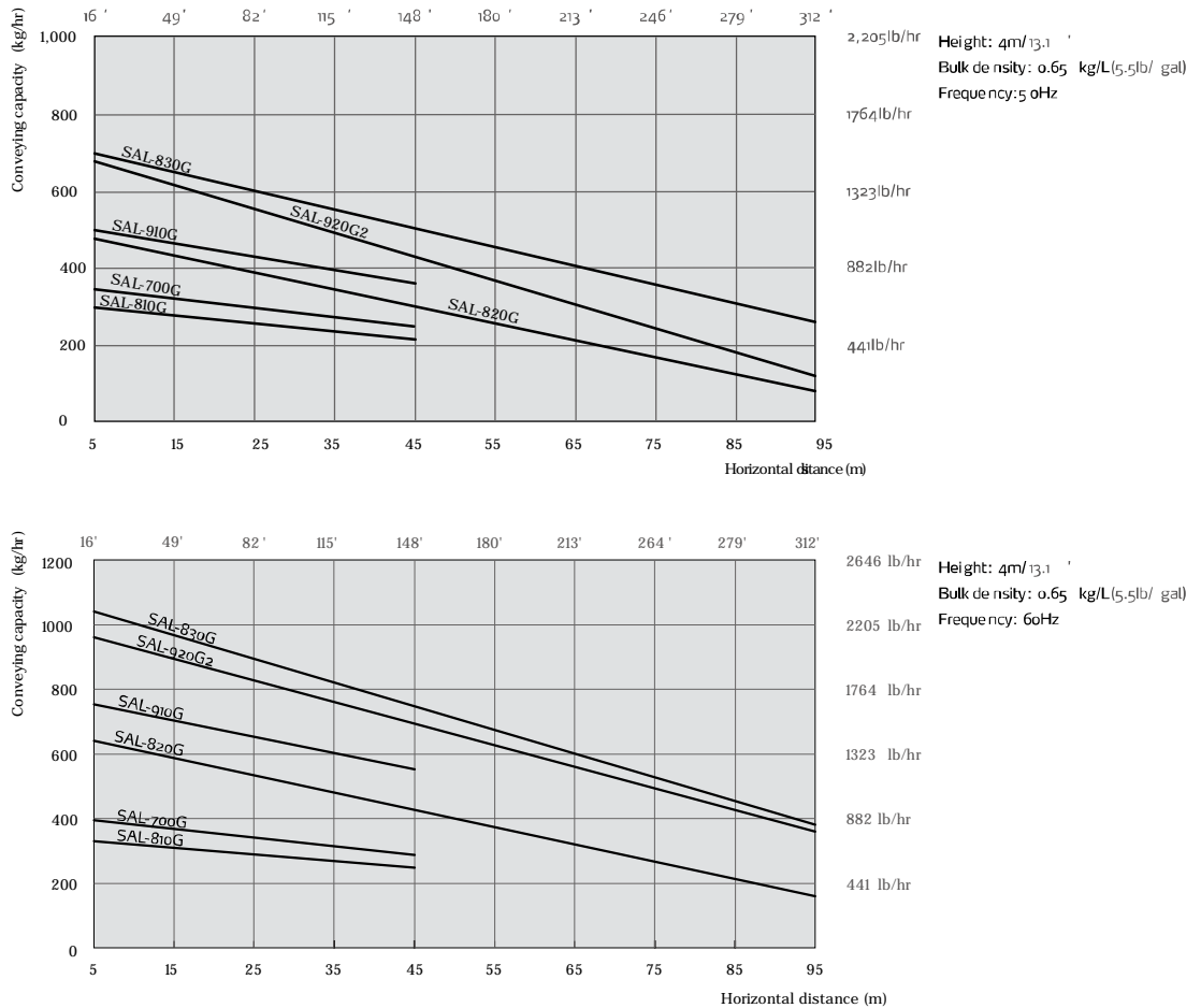
Picture 1-5: Loading Capacity
