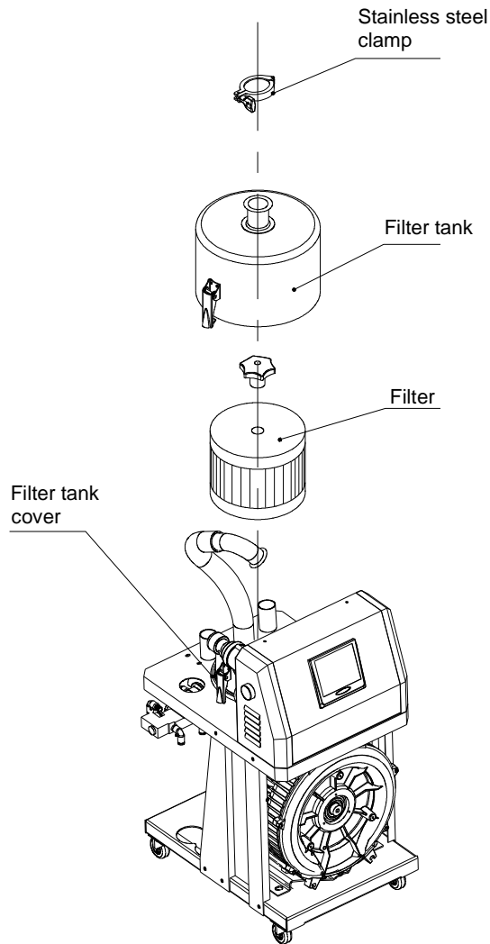
Picture 6-2: Filter Barrel Cleaning Diagram
