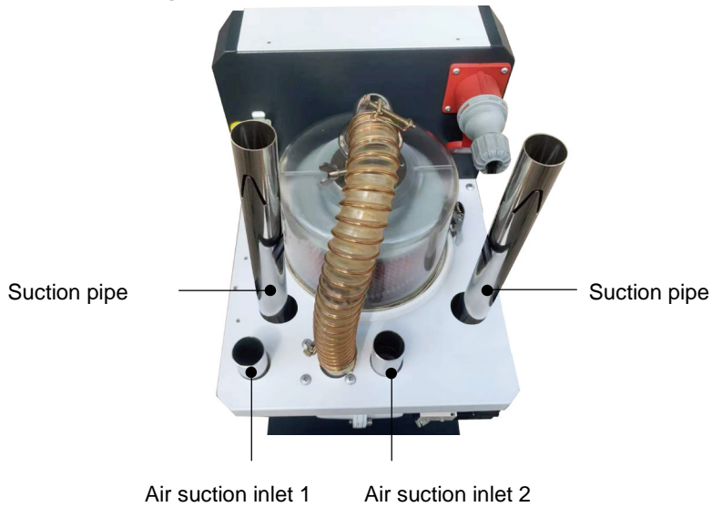
Picture 3-1: Air Suction Inlet
