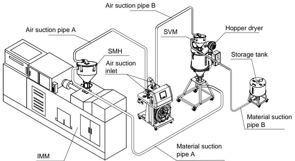
Picture 3-2: Installation Layout 1
