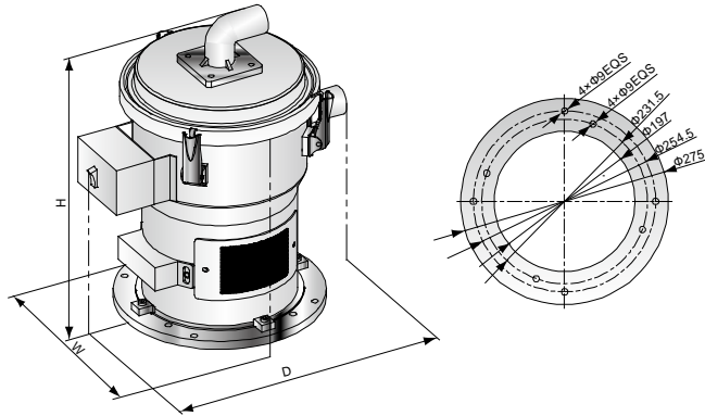
Picture 1-3: SHR External Dimension
