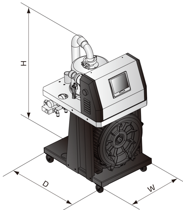
Picture 1-4: SAL-910G External Dimension
