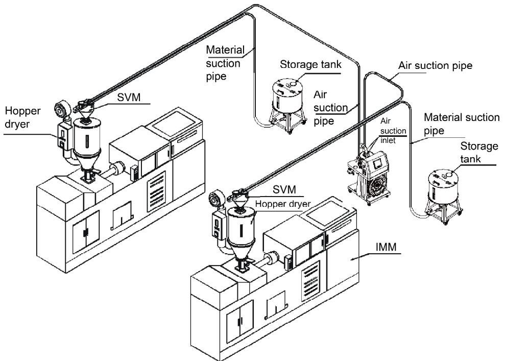
Picture 3-4: Installation Layout 3
