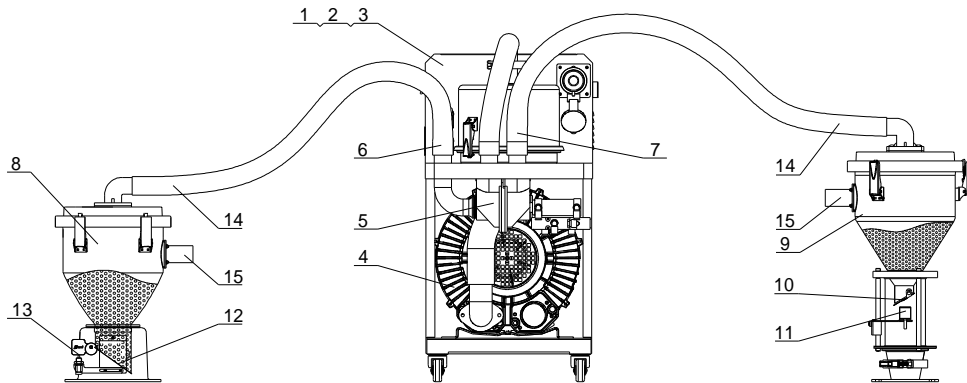
Picture 2-1: Working Principle
