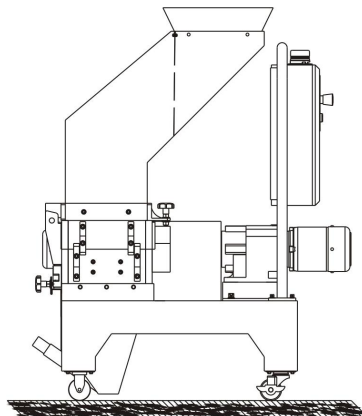
Picture 3-2: Installation Place
