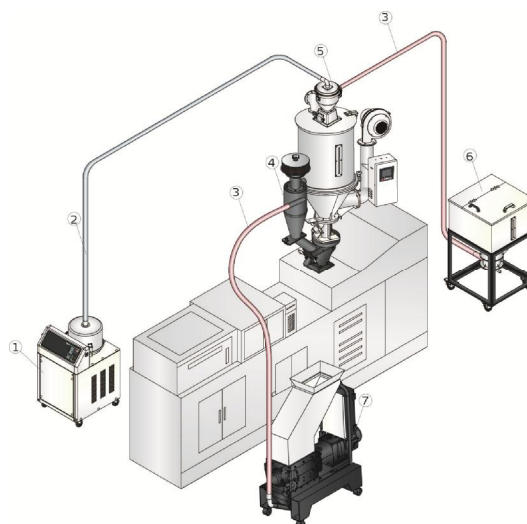
BR Type 30-Sec Instant Recycling
