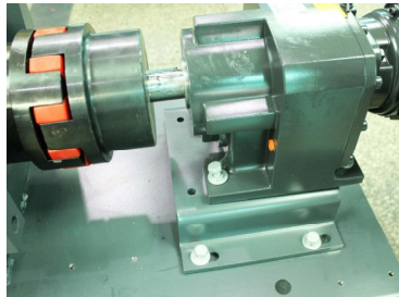
Picture 6-20: Installation of Reduction Gear 2
