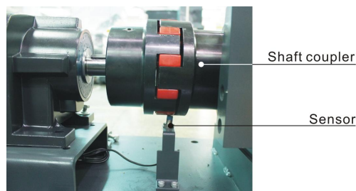
Picture 4-4: Motor Reversed Protection
