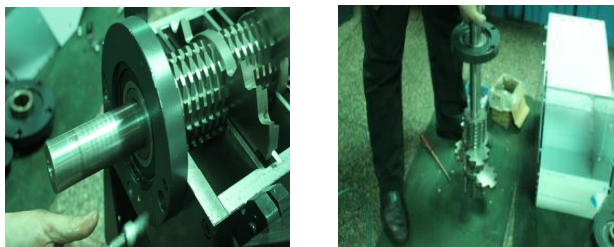
Picture 6-14: Step 2 of Left / Right Bearing Base Dismantlement
