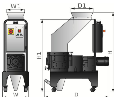
Picture 1-1: Dimensions
