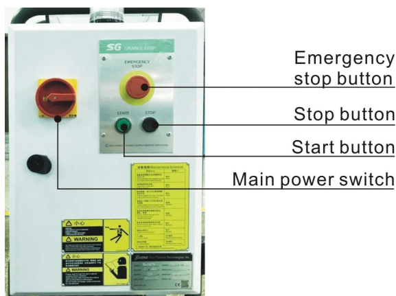
Picture 4-3: START, Emergency Stop and STOP Button
