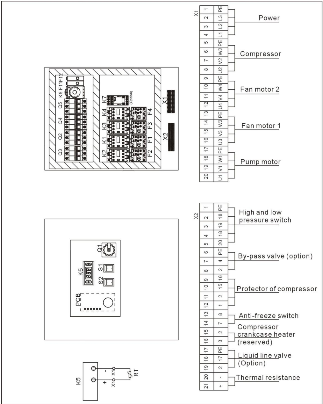
Picture 2-92: Electrical Components Layout (SIC-28A-R2) (230V)
