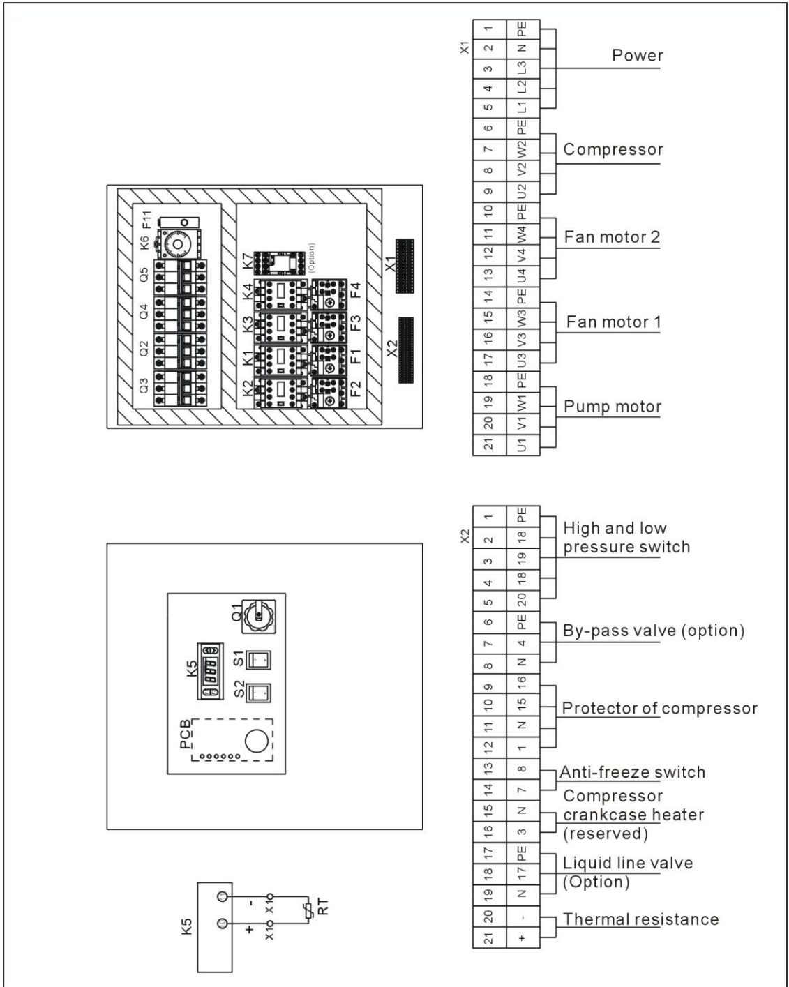
Picture 2-51: Electrical Components Layout (SIC-28A-R2) (400V)
