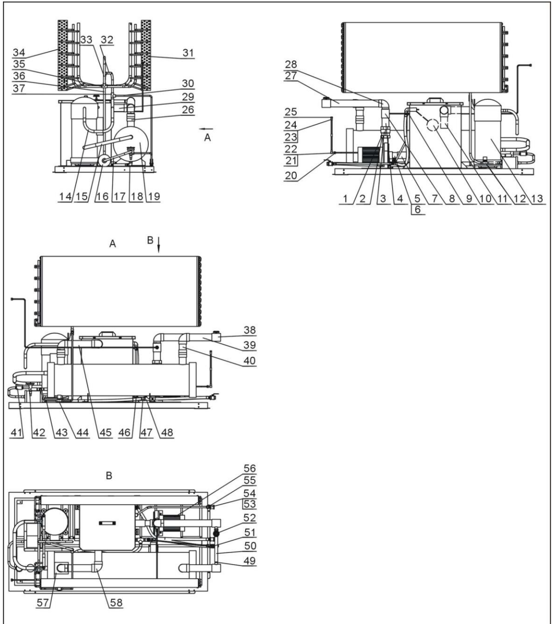
Picture 2-15: Water System & Refrigerant system Diagram
