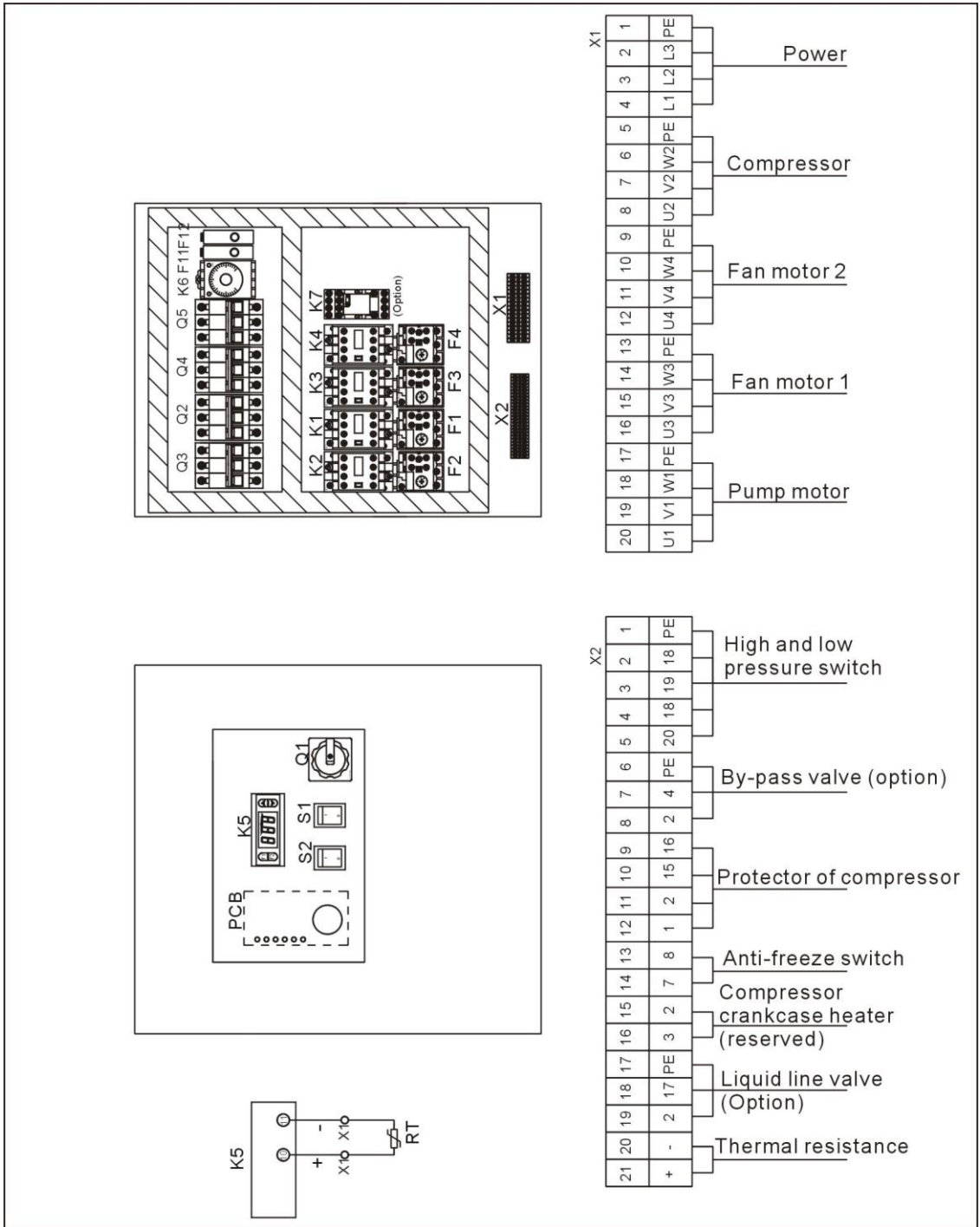
Picture 2-86: Electrical Components Layout (SIC-18A-R2) (230V)
