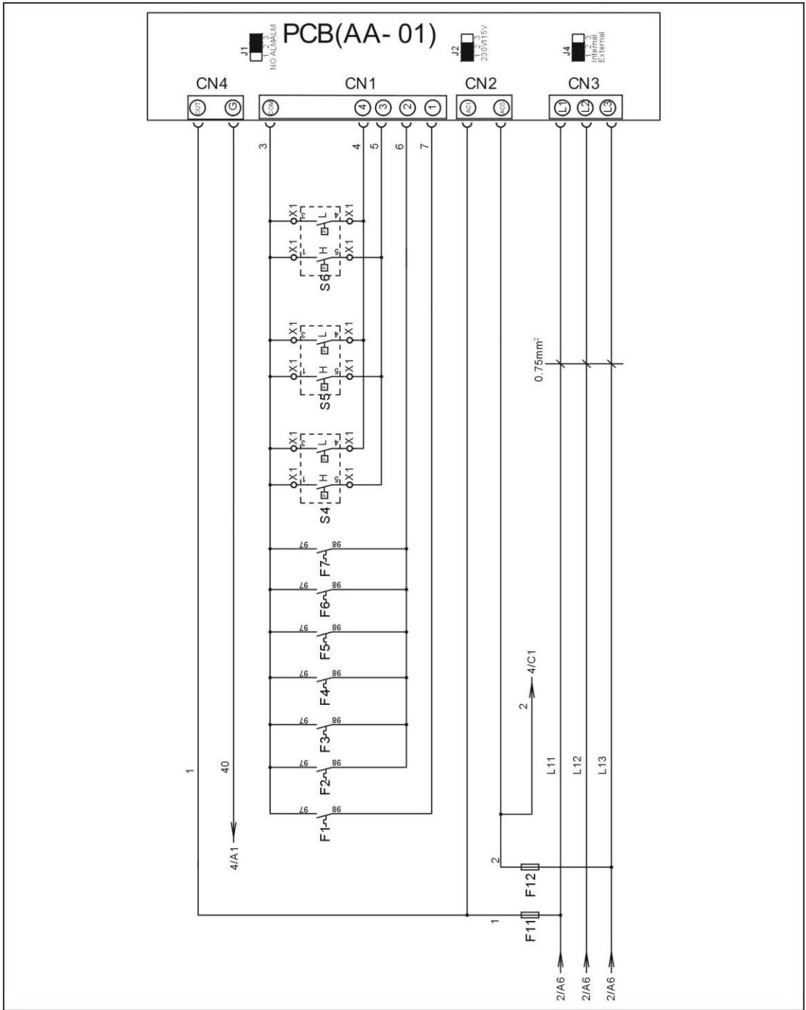
Picture 2-114: Control Circuit 1(SIC-114A-R2) (230V)
