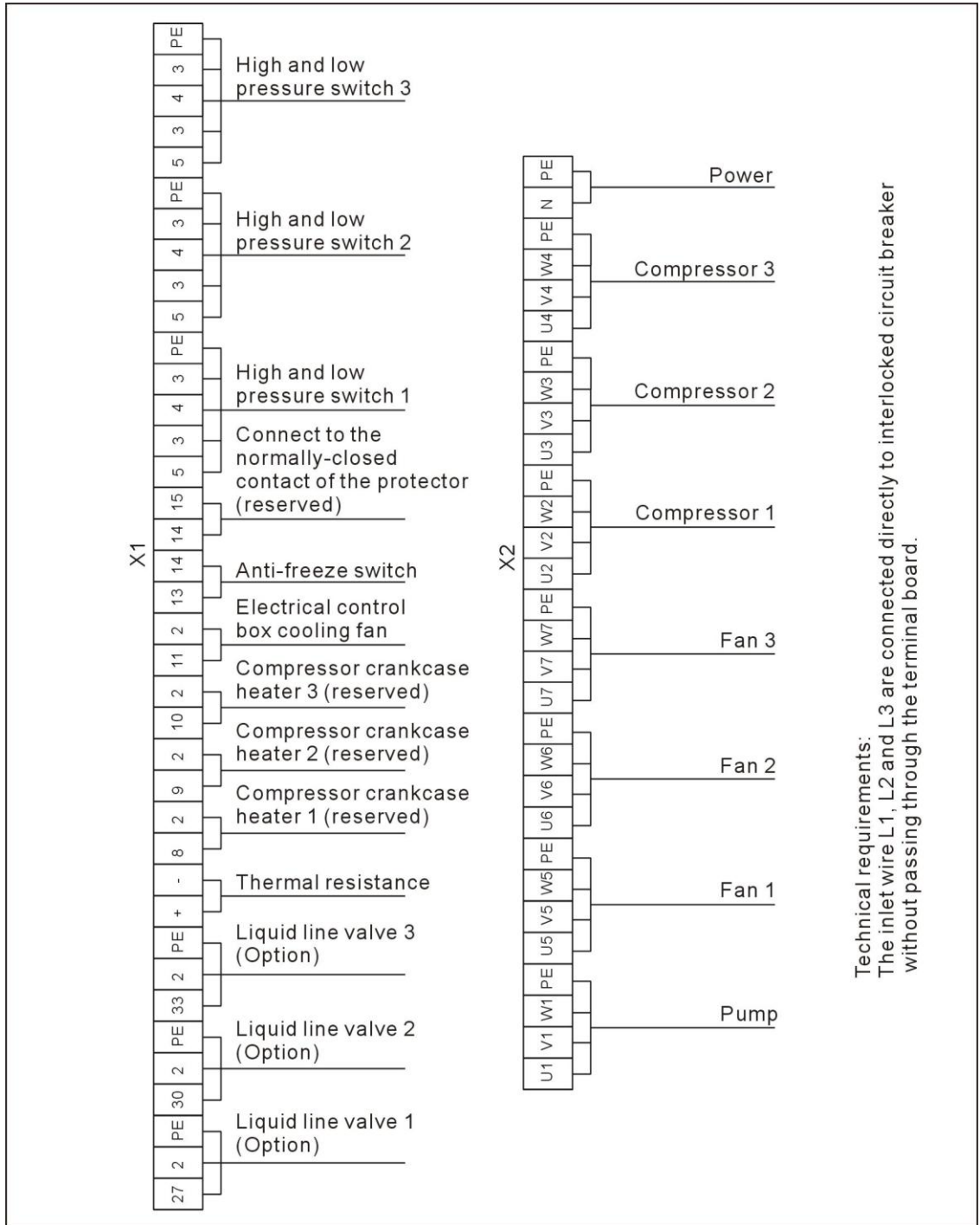
Picture 2-117: Electrical Components Layout 1(SIC-114A-R2) (230V)
