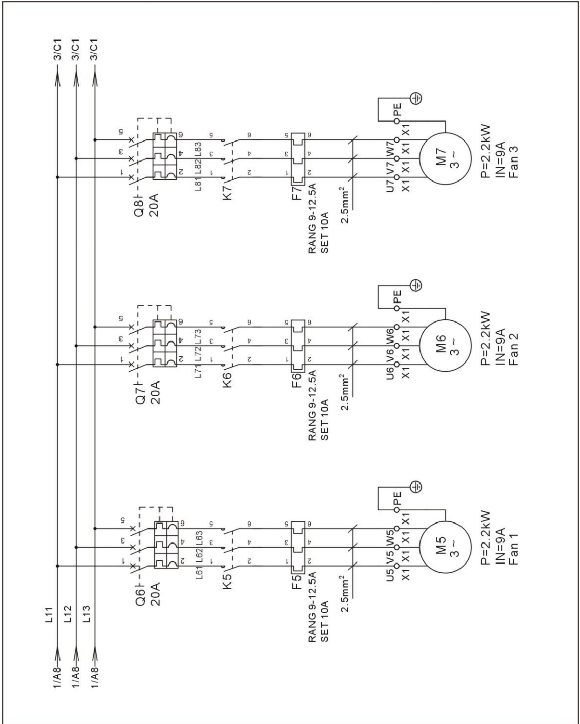
Picture 2-113: Main Electrical Circuit 2(SIC-114A-R2) (230V)
