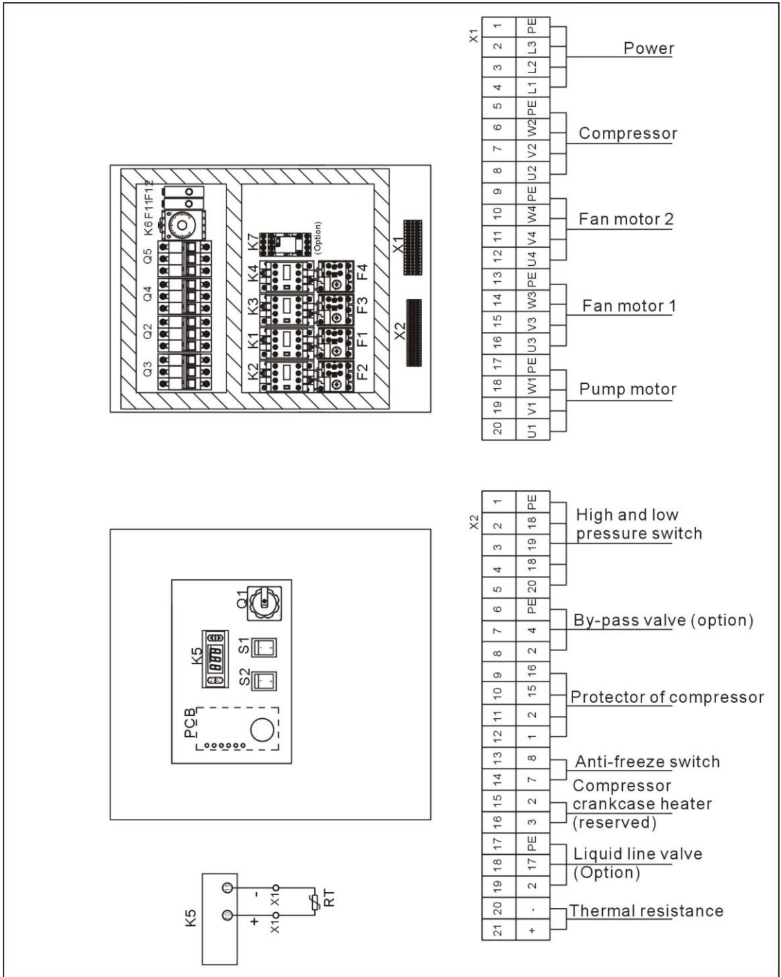
Picture 2-89: Electrical Components Layout (SIC-24A-R2) (230V)
