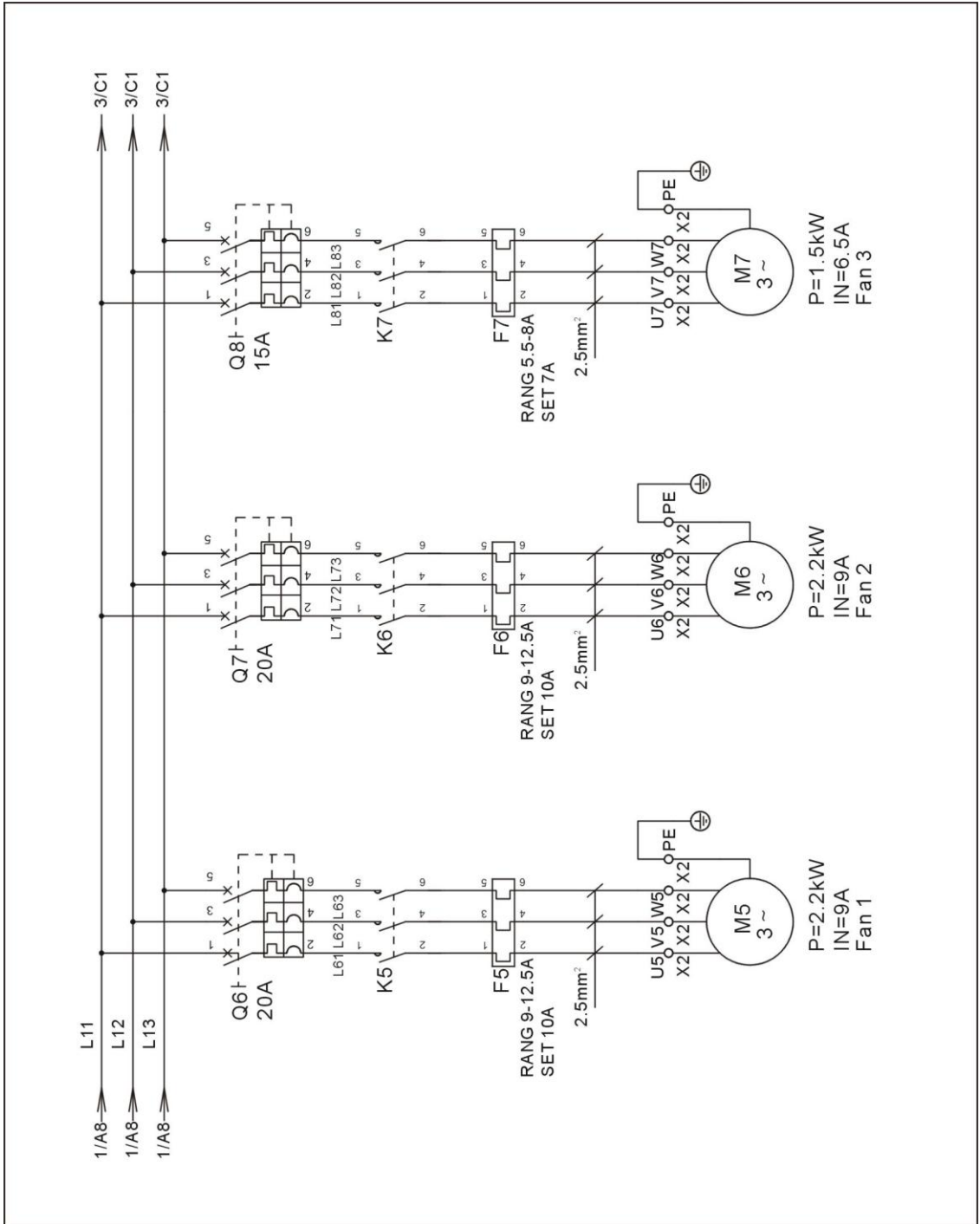
Picture 2-106: Main Electrical Circuit 2(SIC-100A-R2) (230V)
