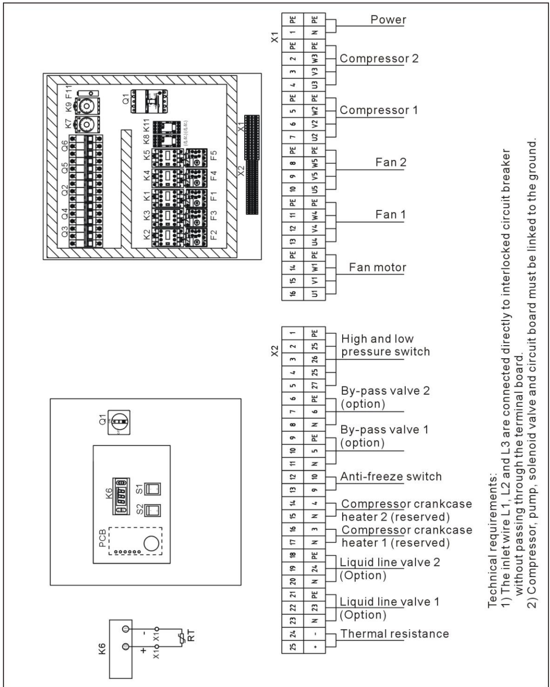
Picture 2-60: Electrical Components Layout (SIC-58A-R2) (400V)
