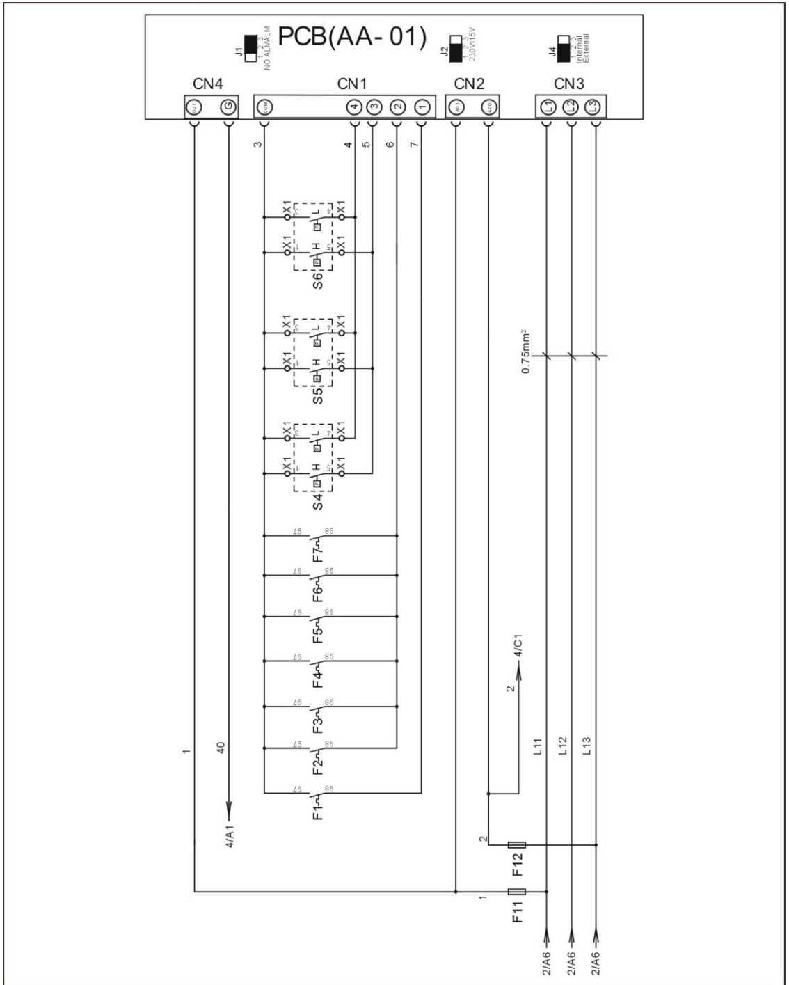
Picture 2-107: Control Circuit 1(SIC-100A-R2) (230V)
