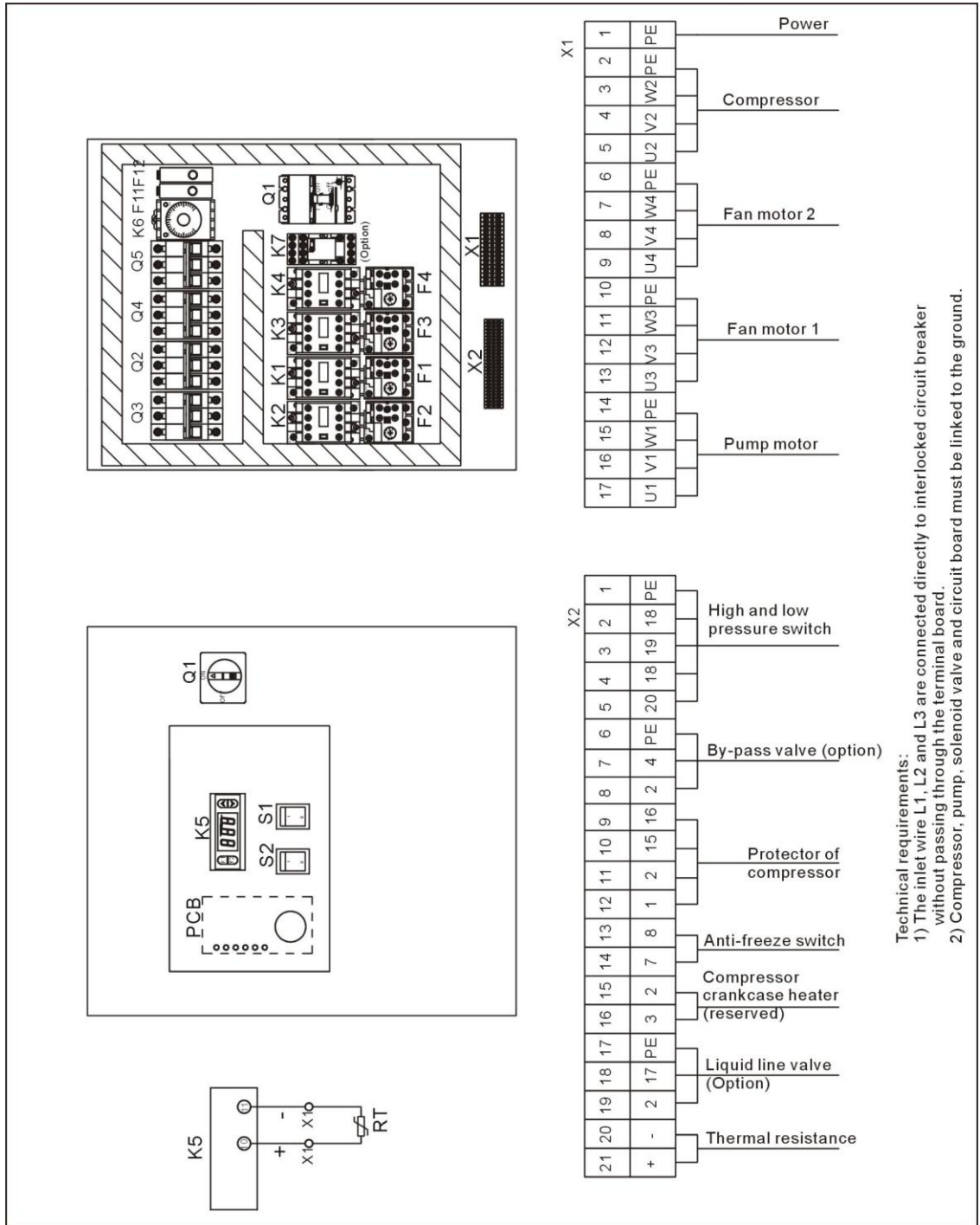
Picture 2-95: Electrical Components Layout (SIC-38A-R2) (230V)
