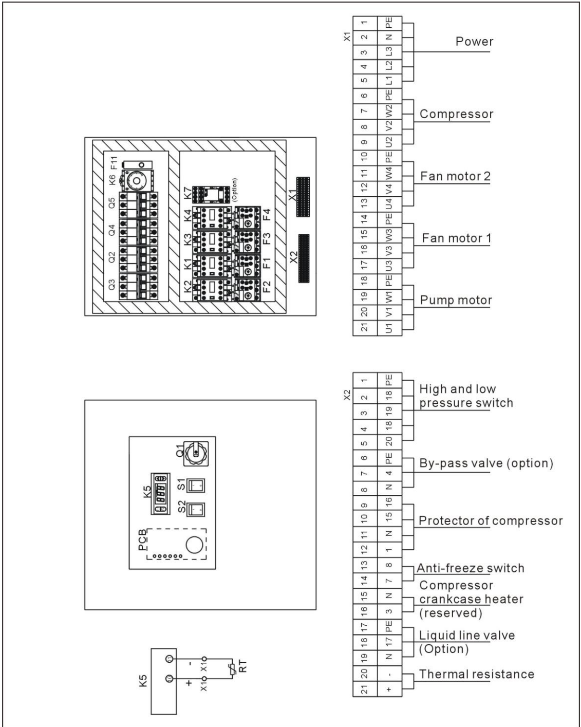
Picture 2-45: Electrical Components Layout (SIC-18A-R2) (400V)
