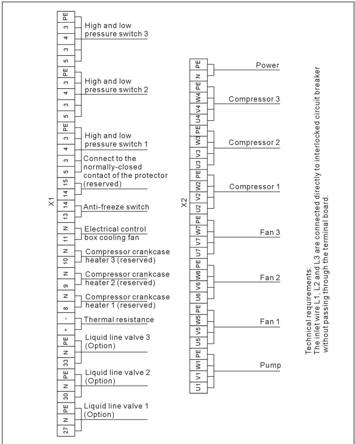
Picture 2-69: Electrical Components Layout 1(SIC-100A-R2) (400V)
