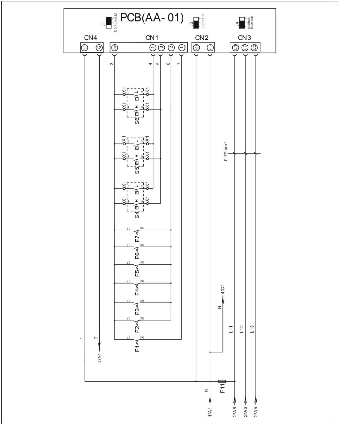
Picture 2-66: Control Circuit 1(SIC-100A-R2) (400V)
