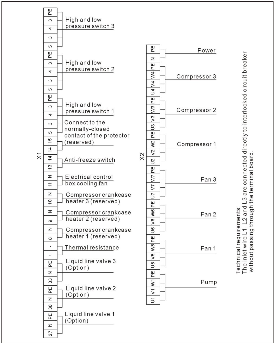
Picture 2-76: Electrical Components Layout 1(SIC-114A-R2) (400V)
