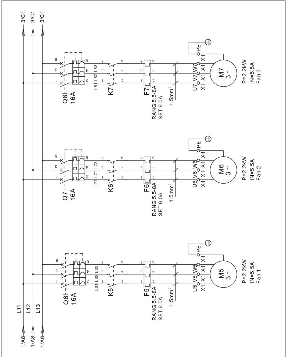
Picture 2-72: Main Electrical Circuit 2(SIC-114A-R2) (400V)
