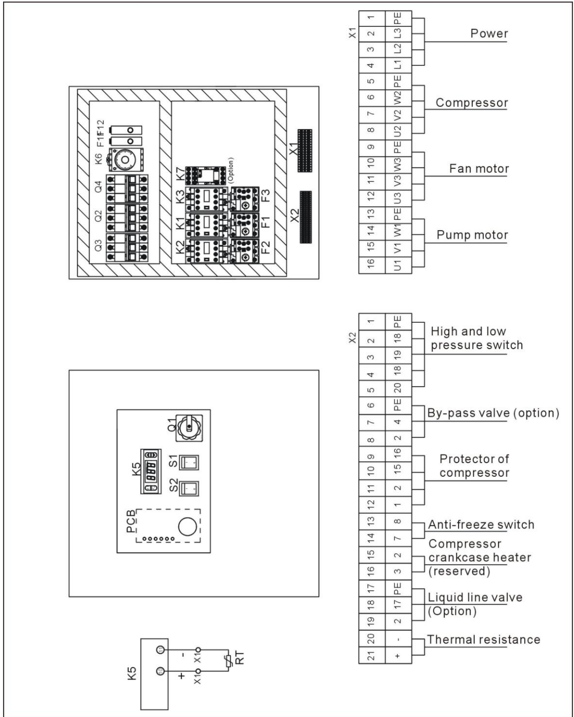
Picture 2-80: Electrical Components Layout (SIC-7.5A-R2) (230V)
