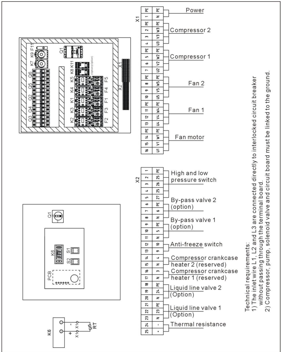
Picture 2-57: Electrical Components Layout (SIC-48A-R2) (400V)
