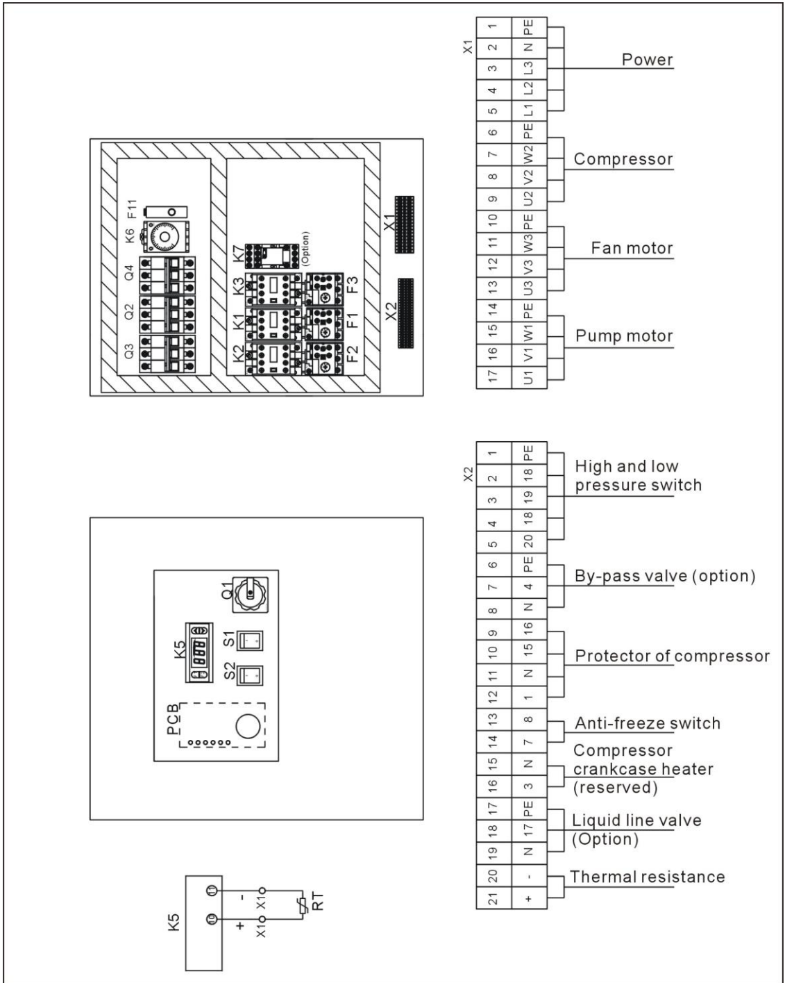
Picture 2-42: Electrical Components Layout (SIC-12A-R2) (400V)
