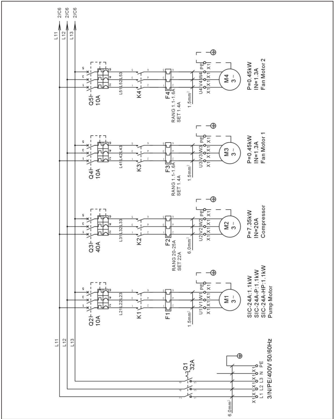
Picture 2-46: Main Electrical Circuit (SIC-24A-R2) (400V)
