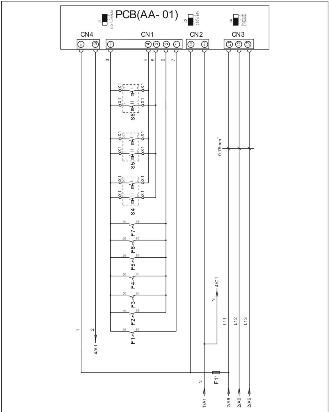
Picture 2-73: Control Circuit 1(SIC-114A-R2) (400V)
