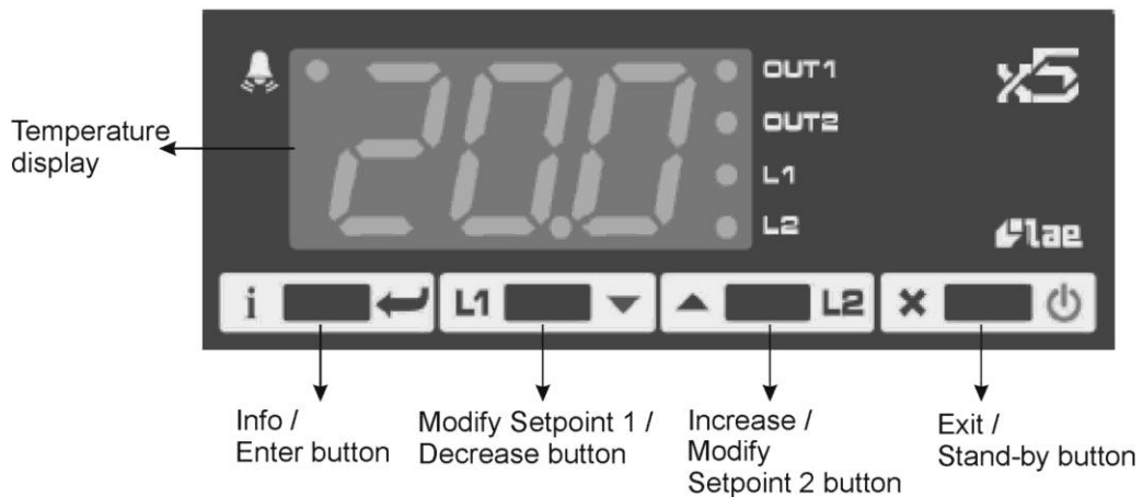
Picture 4-3: Thermostat
