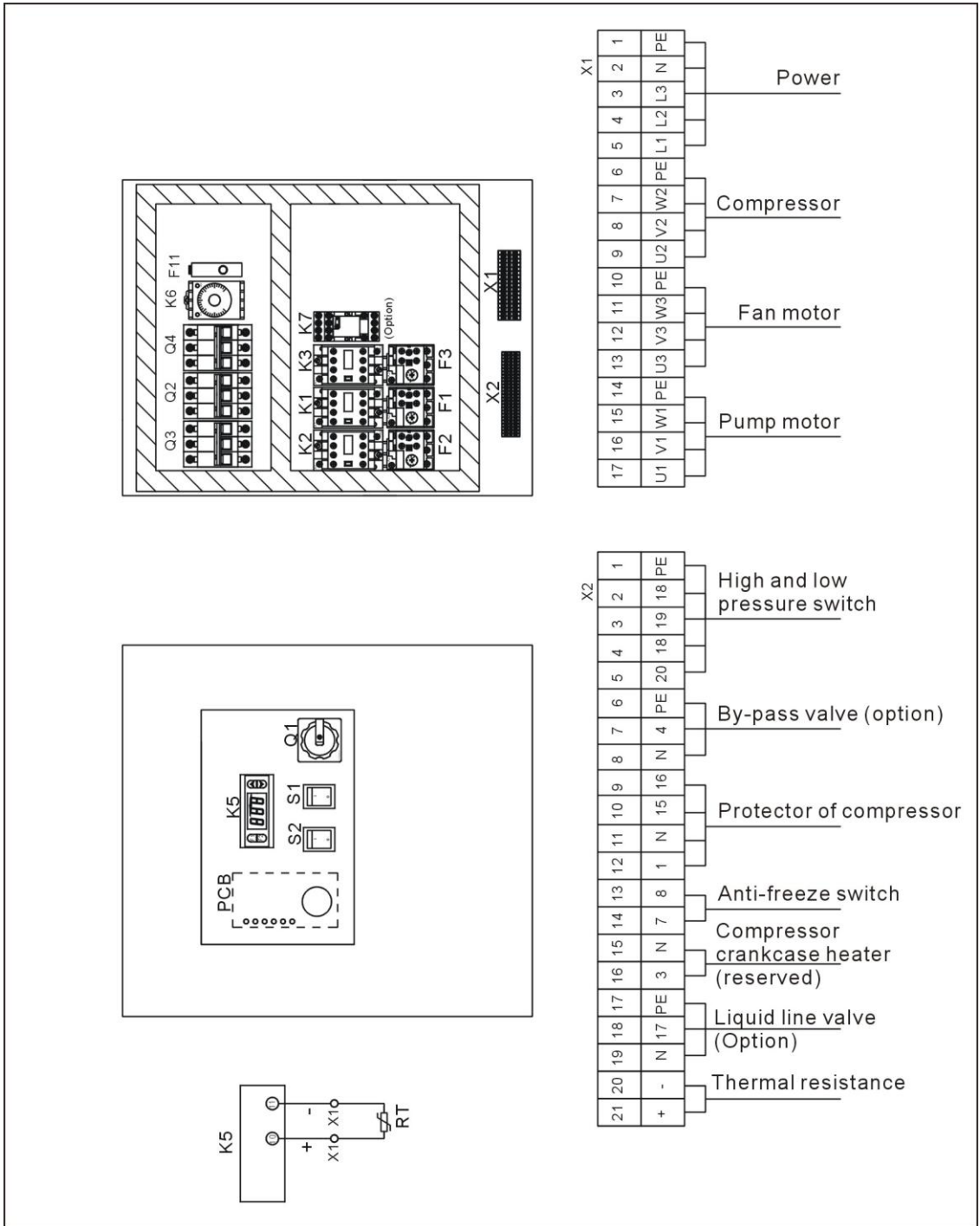
Picture 2-39: Electrical Components Layout (SIC-7.5A-R2) (400V)
