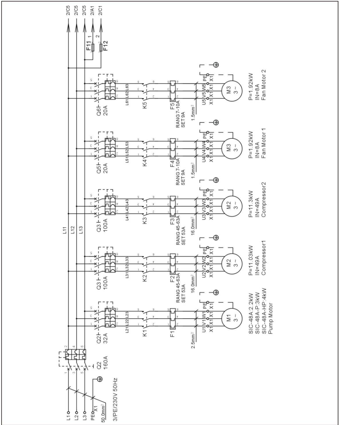
Picture 2-102: Main Electrical Circuit (SIC-75A-R2) (230V)
