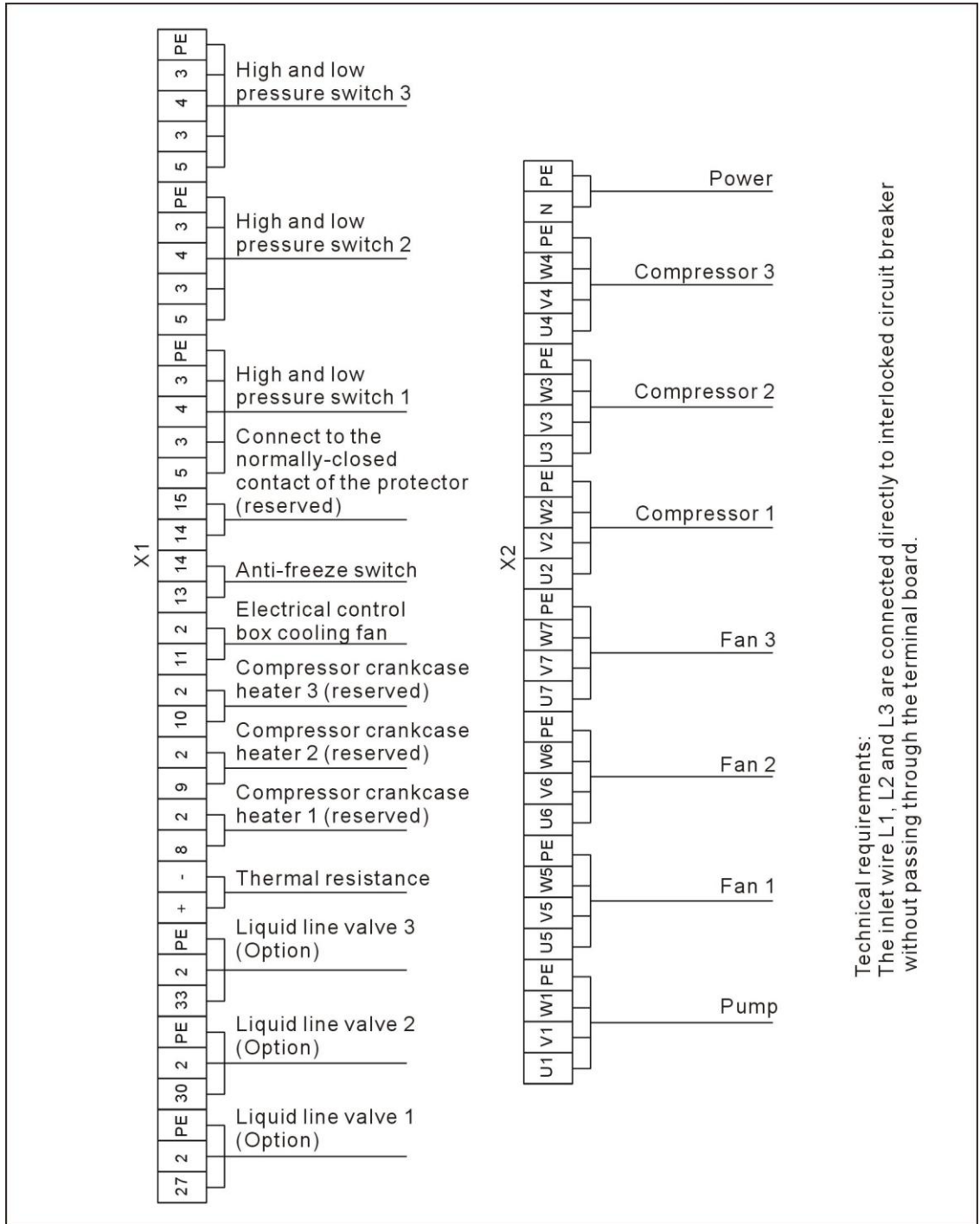
Picture 2-110: Electrical Components Layout 1(SIC-100A-R2) (230V)
